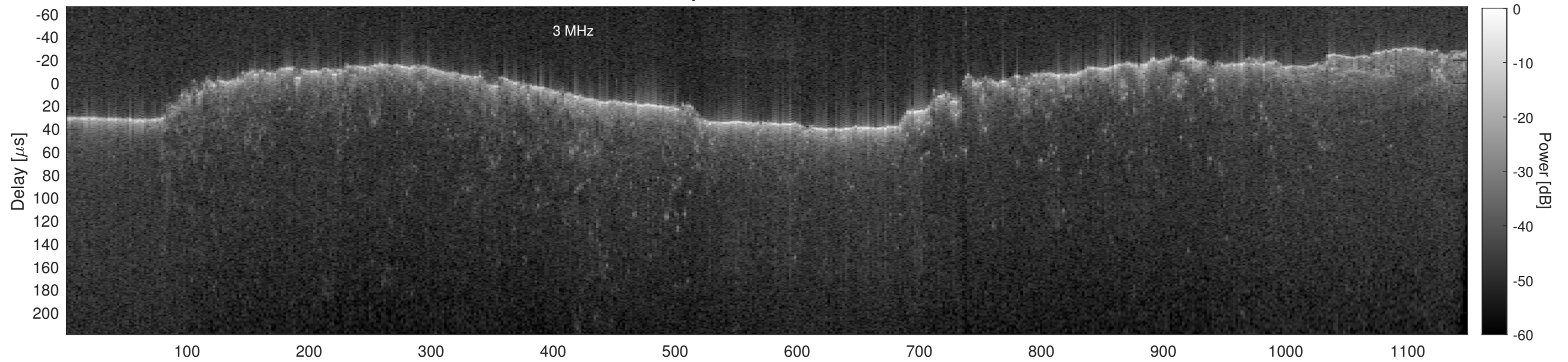
Orbit 17409, Cluttergram
