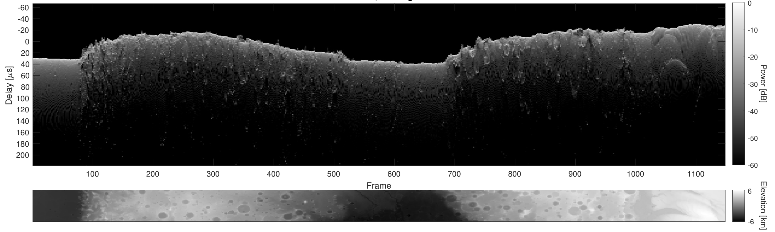
Orbit 17409, Cluttergram
