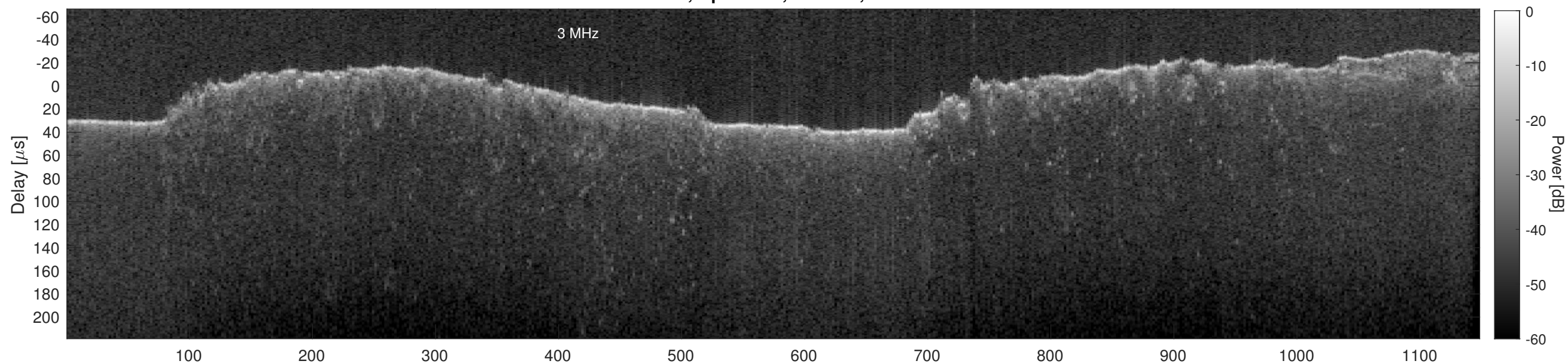
Orbit 17409, Cluttergram
