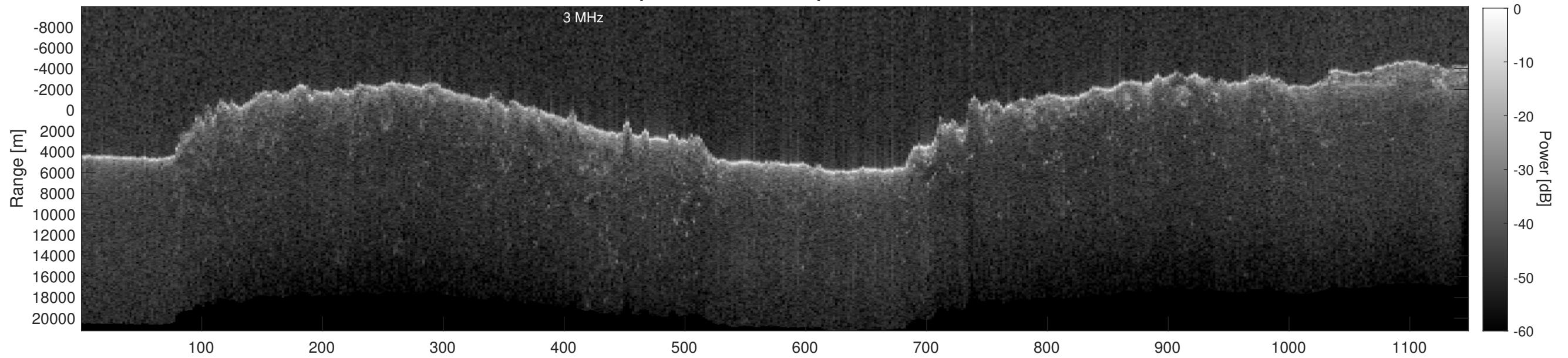
Orbit 17409, Depth-Corrected Cluttergram
