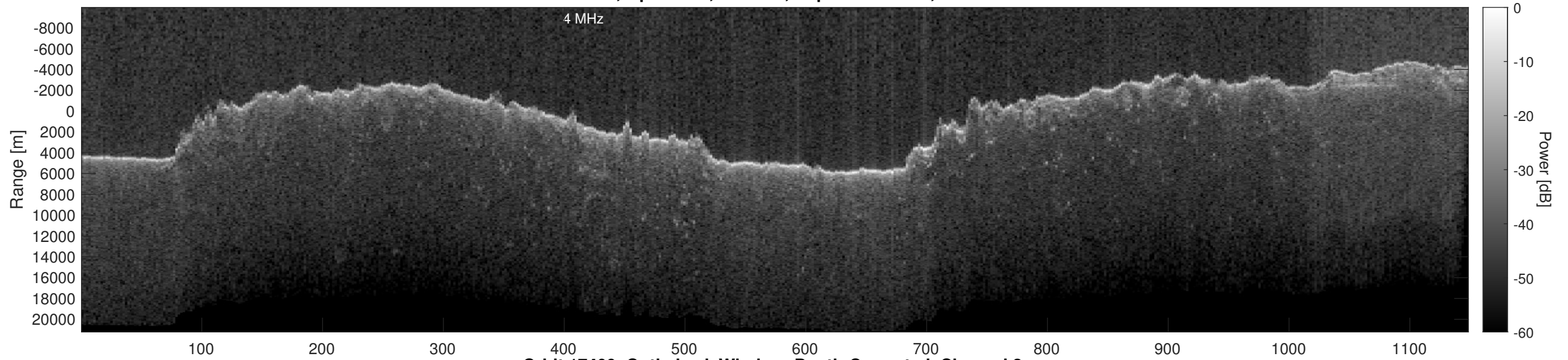
Orbit 17409, Optimized, Window, Depth-Corrected, Channel 2
