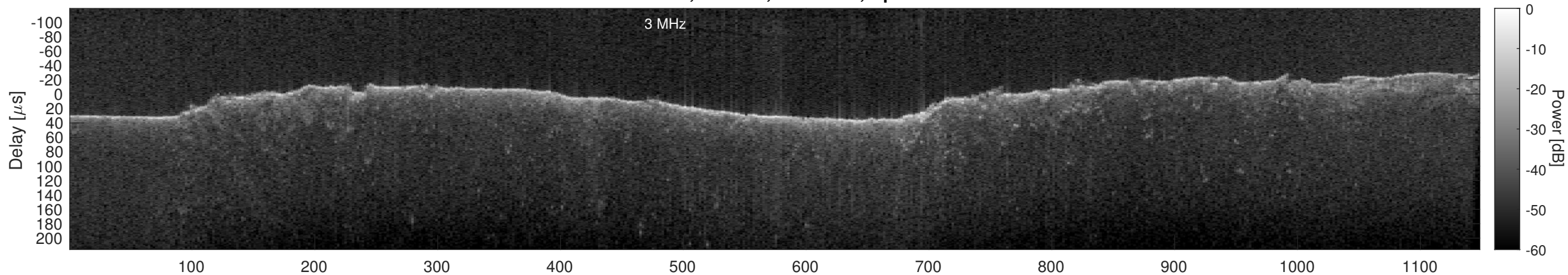
Orbit 17416, Cluttergram
