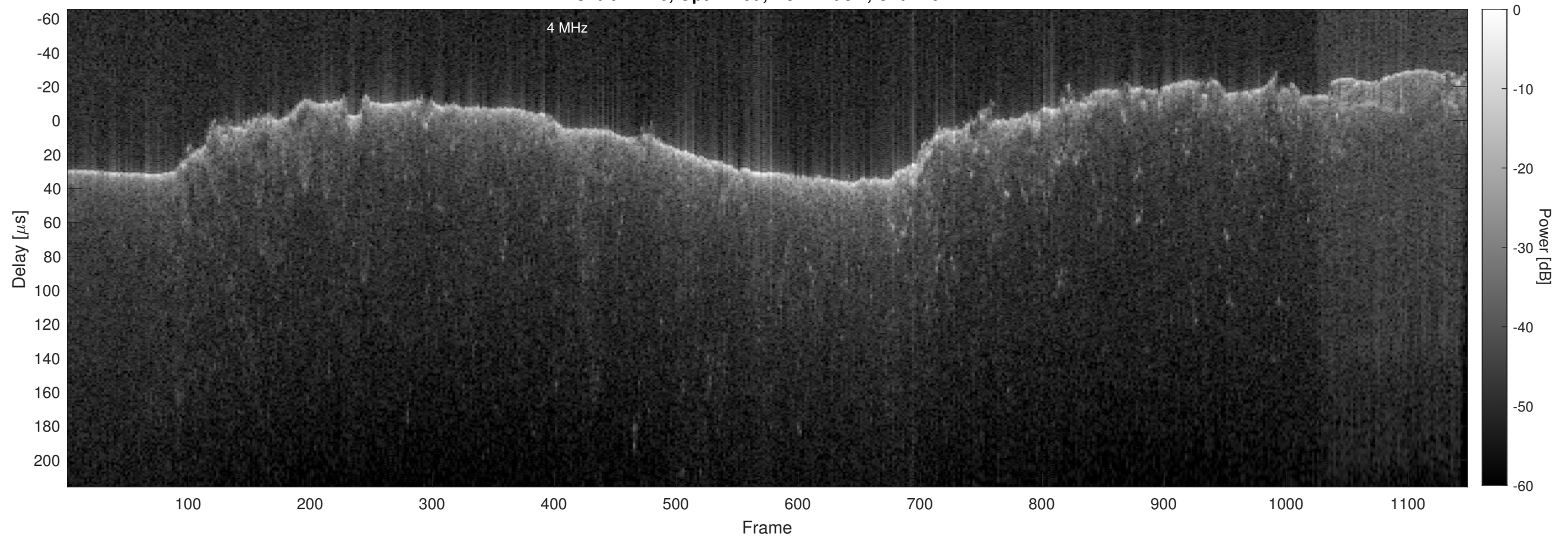
Orbit 17416, Optimized, No Window, Channel 2
