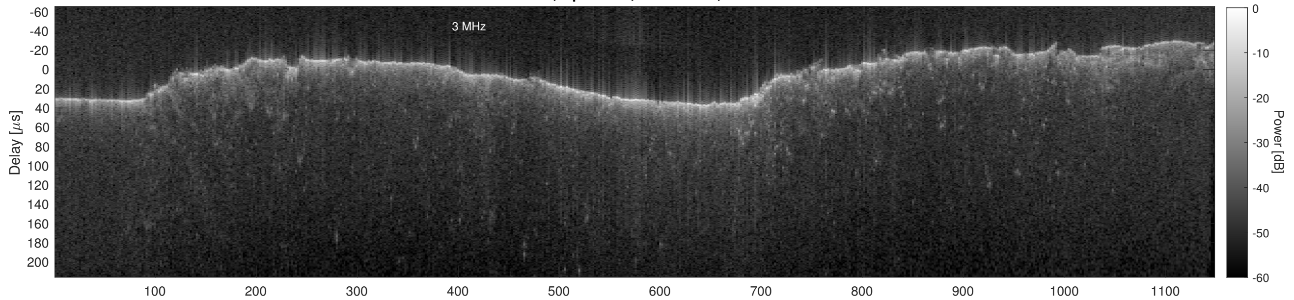
Orbit 17416, Cluttergram
