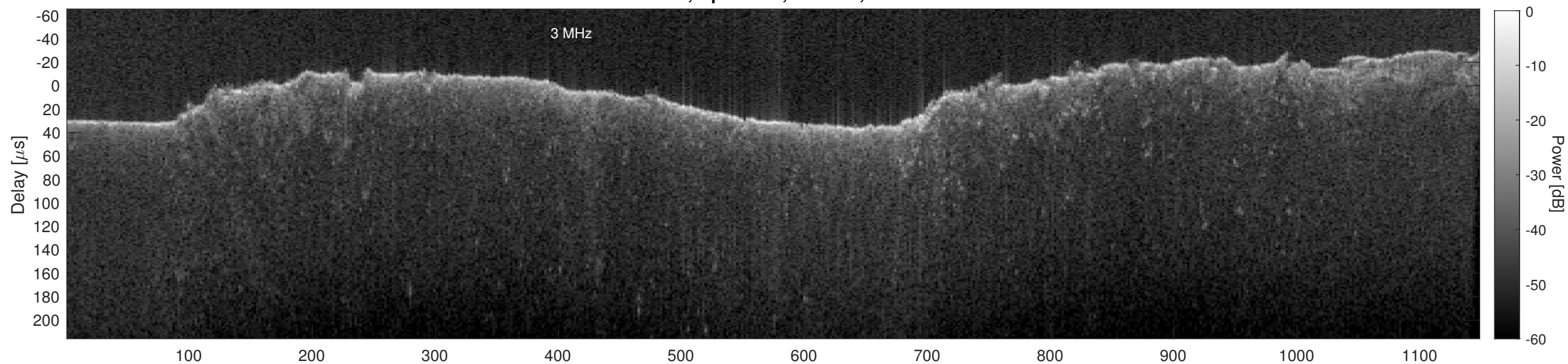
Orbit 17416, Cluttergram
