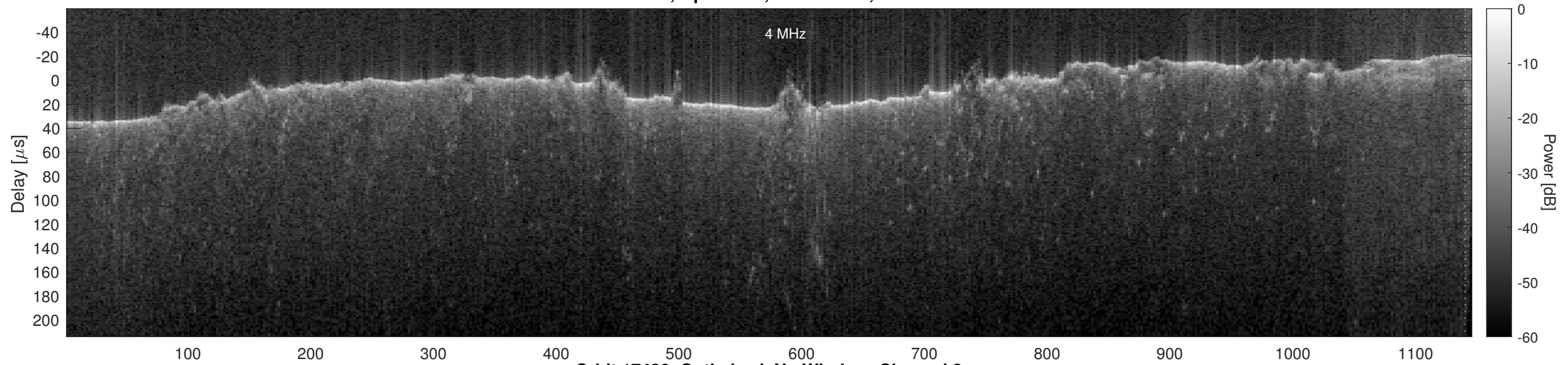
Orbit 17430, Optimized, No Window, Channel 2
