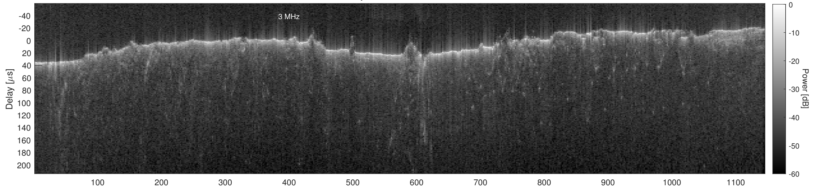
Orbit 17430, Cluttergram
