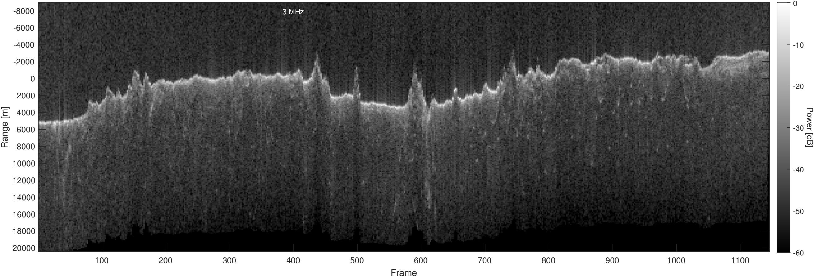
Orbit 17430, Optimized, Window, Depth-Corrected, Channel 2
