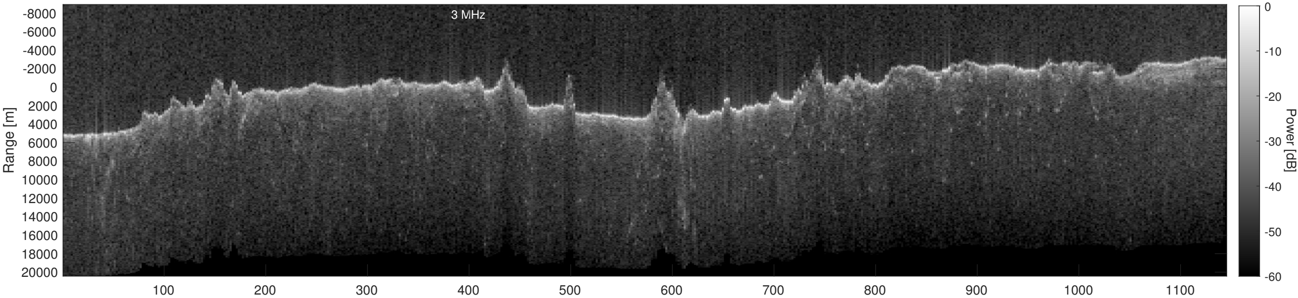
Orbit 17430, Depth-Corrected Cluttergram
