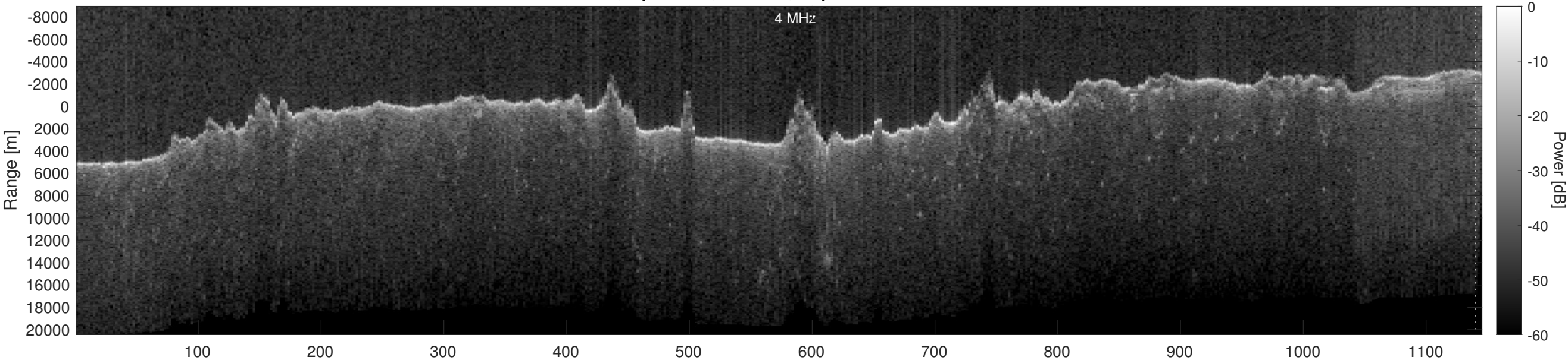
Orbit 17430, Optimized, Window, Depth-Corrected, Channel 2
