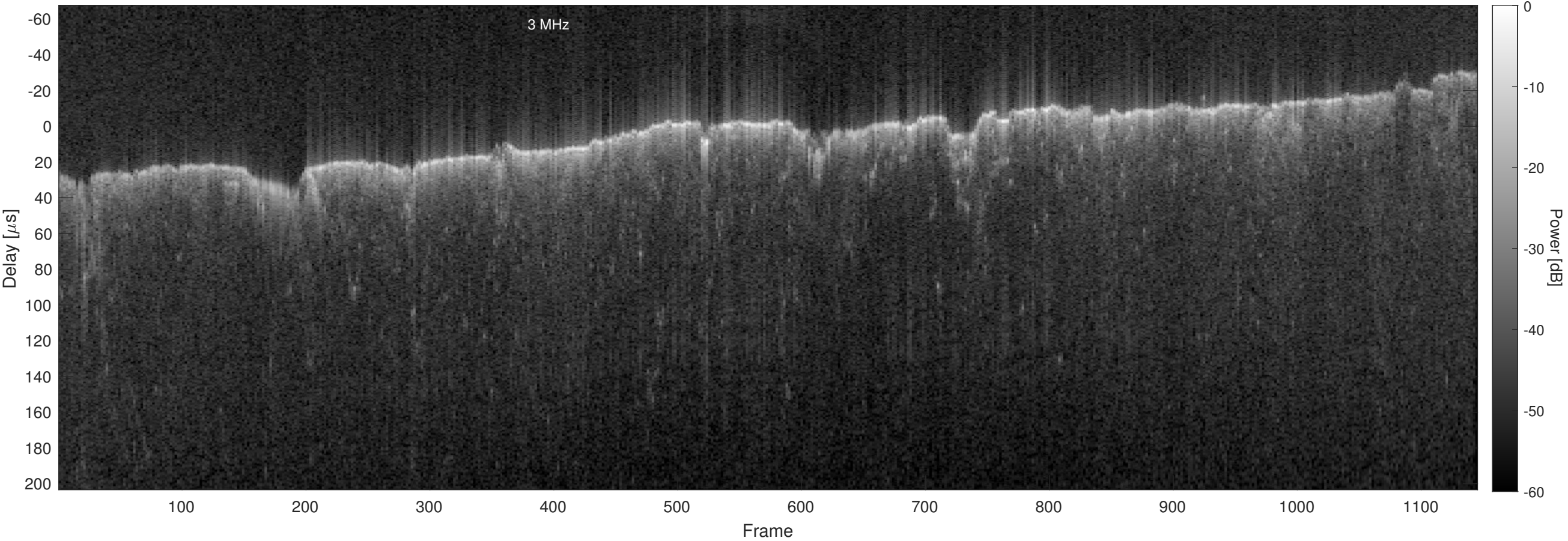
Orbit 17431, Chapman, No Window, Channel 2
