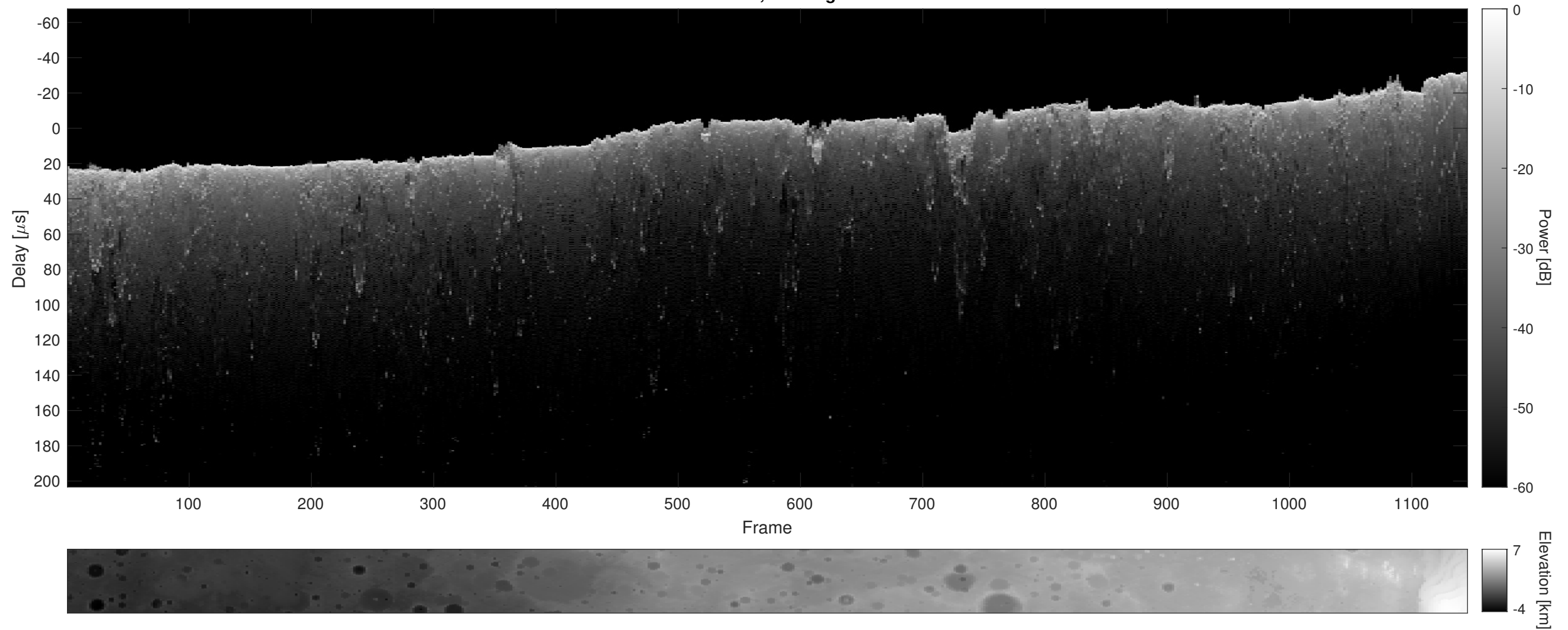
Orbit 17431, Cluttergram
