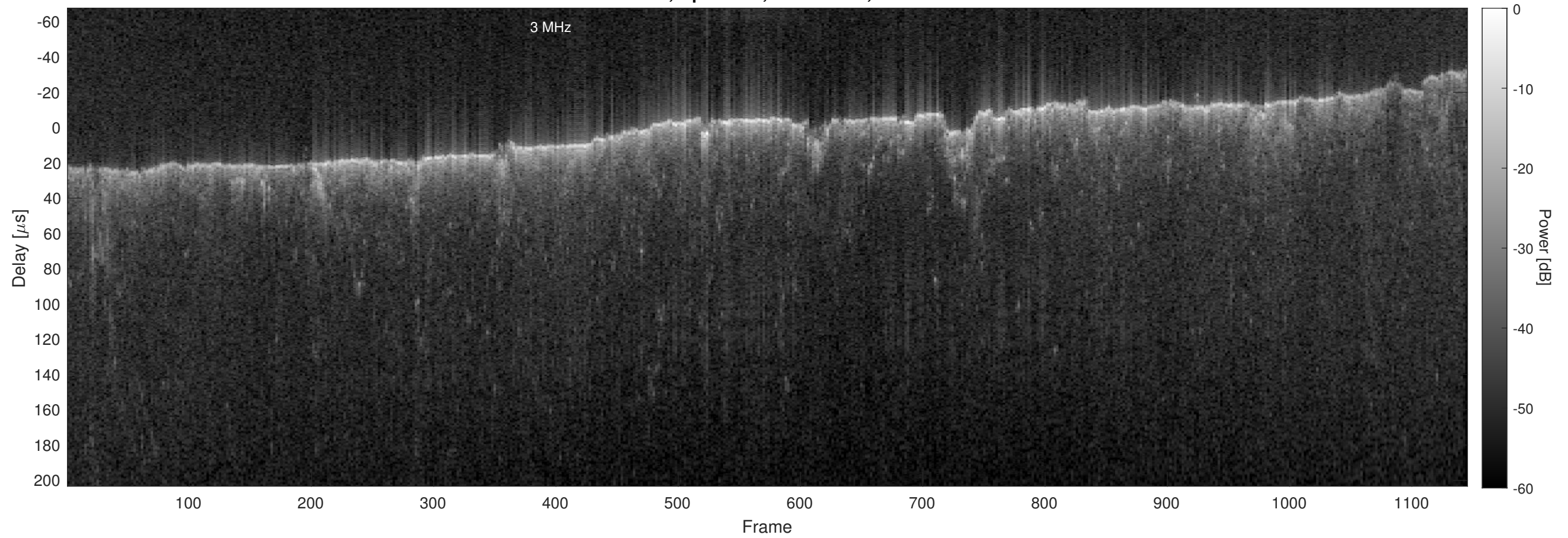
Orbit 17431, Optimized, No Window, Channel 2
