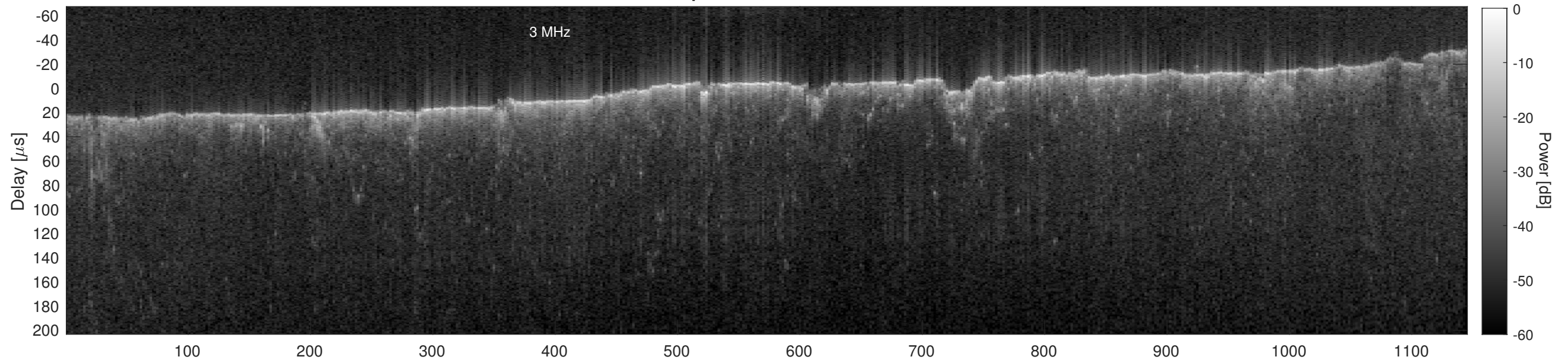
Orbit 17431, Cluttergram
