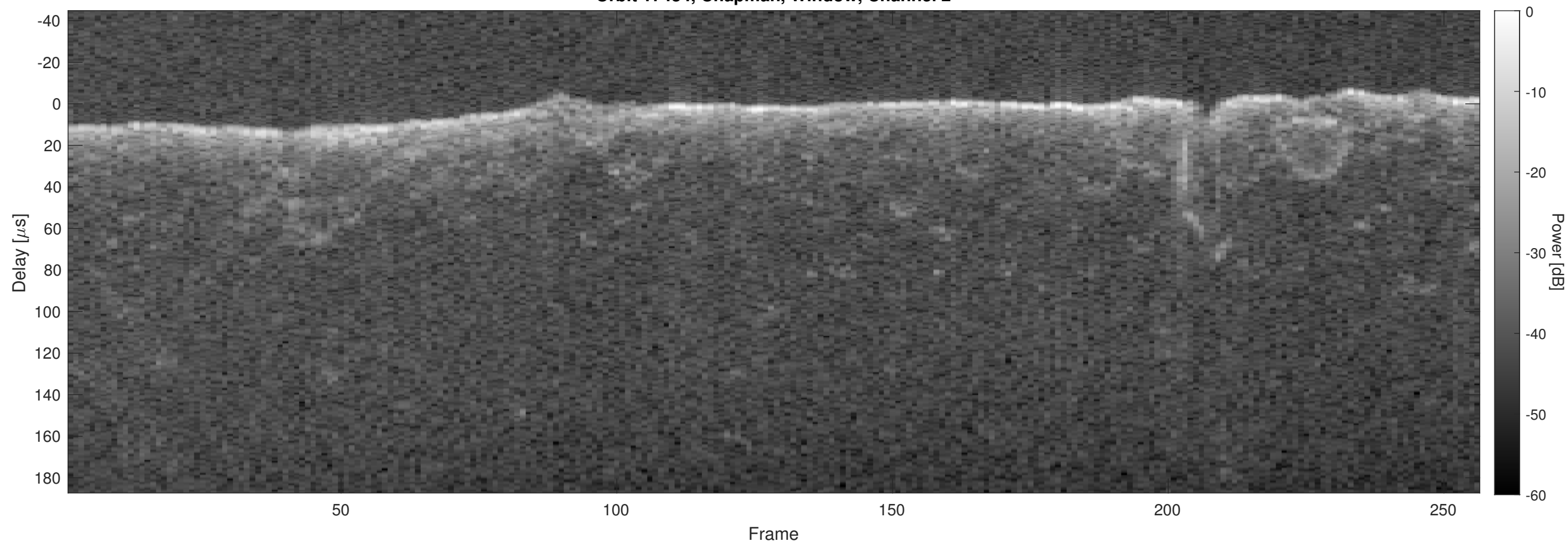
Orbit 17434, Chapman, Window, Channel 2
