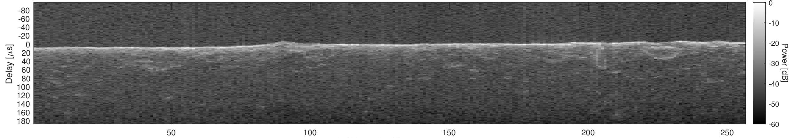
Orbit 17434, Cluttergram
