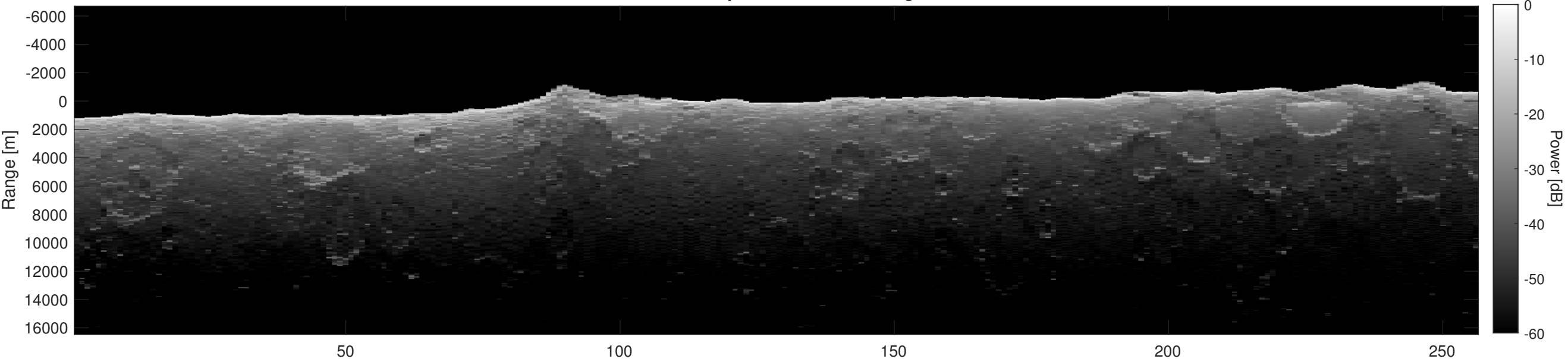
Orbit 17434, Depth-Corrected Cluttergram
