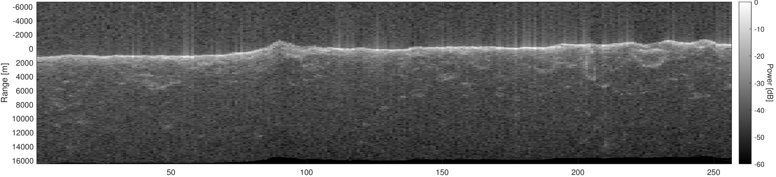
Orbit 17434, Optimized, No Window, Depth-Corrected, Channel 2
