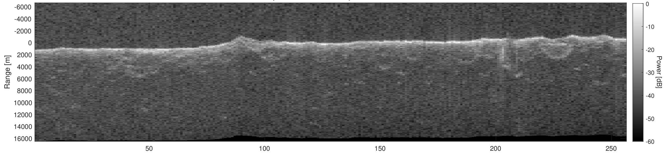
Orbit 17434, Depth-Corrected Cluttergram
