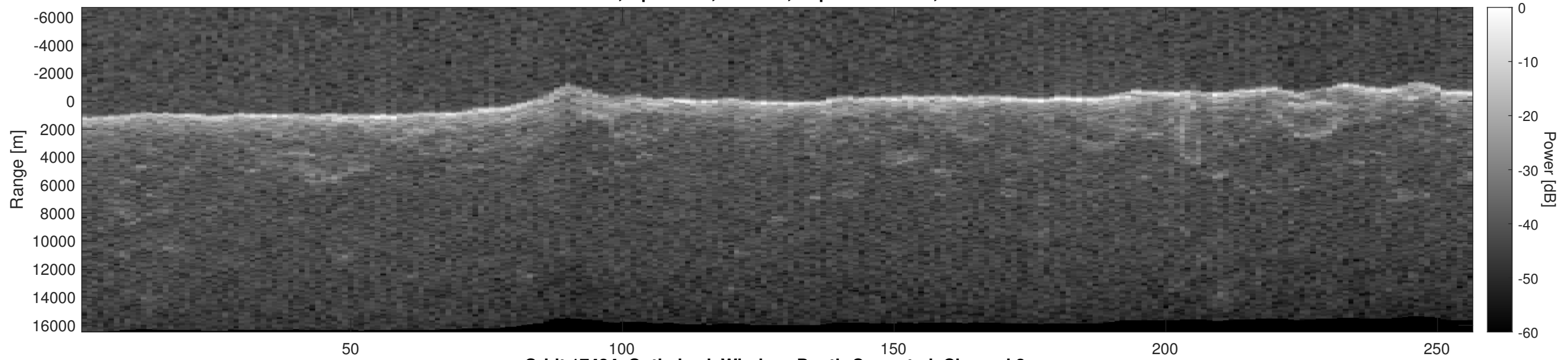
Orbit 17434, Optimized, Window, Depth-Corrected, Channel 2
