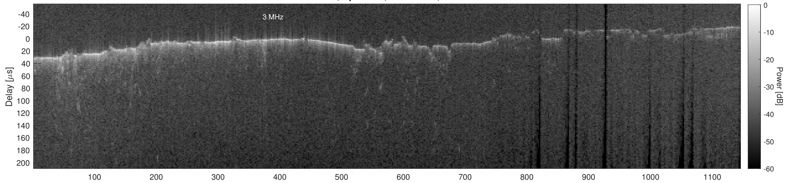
Orbit 17437, Cluttergram
