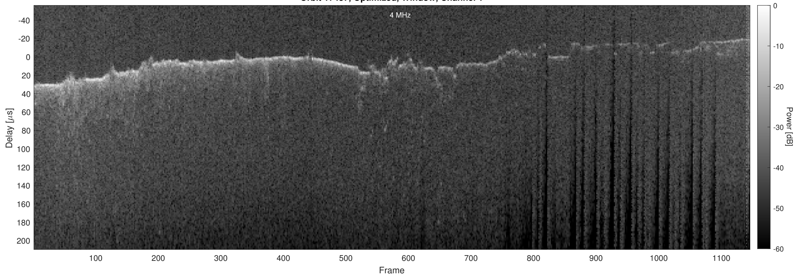
Orbit 17437, Optimized, Window, Channel 2
