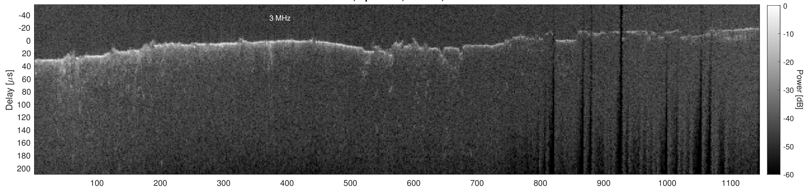
Orbit 17437, Cluttergram
