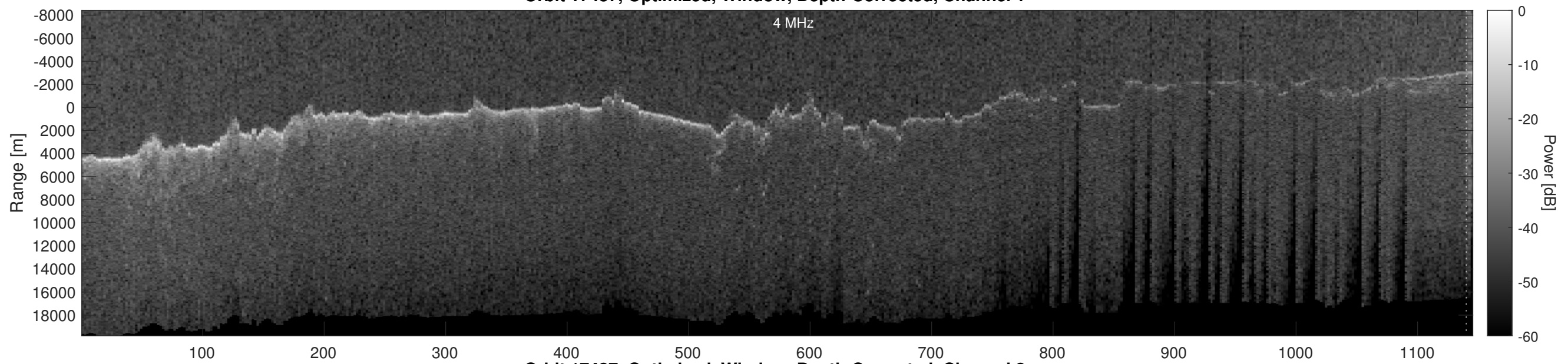
Orbit 17437, Optimized, Window, Depth-Corrected, Channel 2
