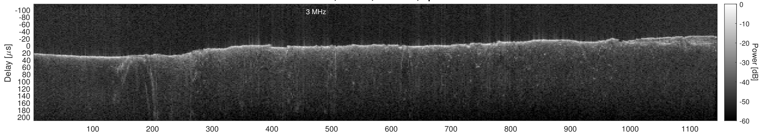
Orbit 17440, Cluttergram
