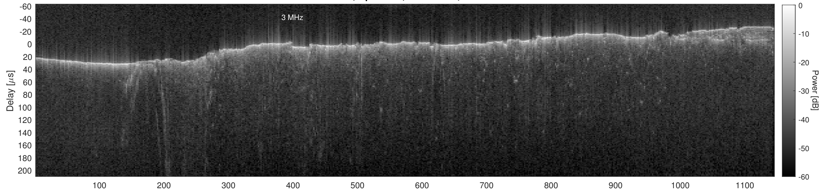
Orbit 17440, Cluttergram
