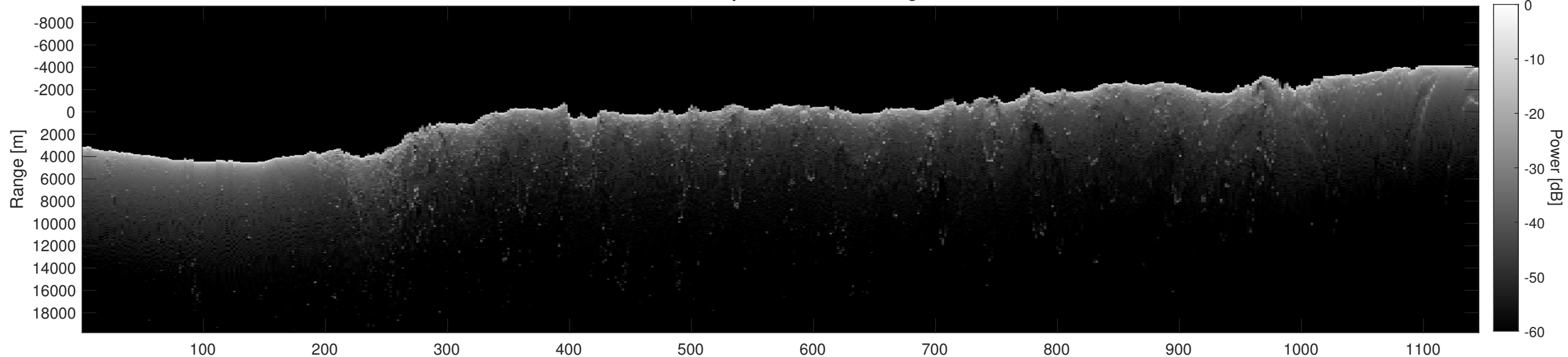
Orbit 17440, Depth-Corrected Cluttergram
