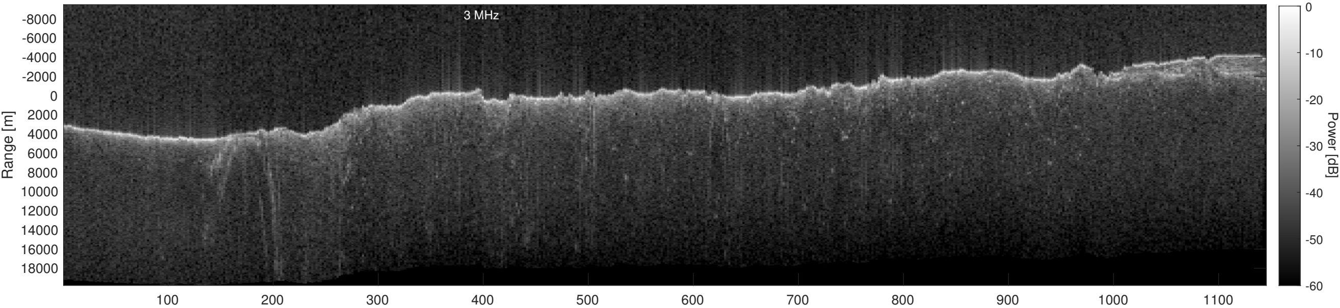
Orbit 17440, Depth-Corrected Cluttergram
