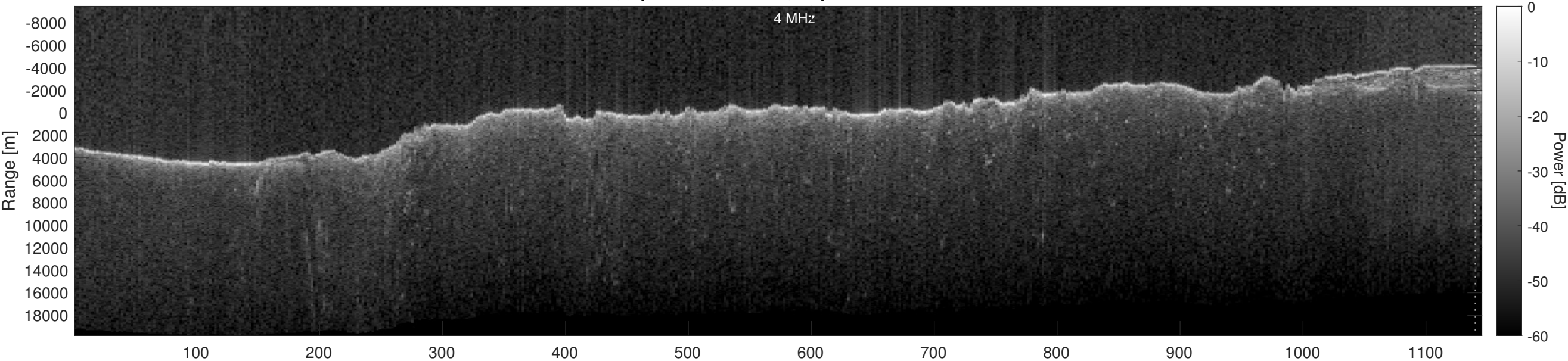
Orbit 17440, Optimized, Window, Depth-Corrected, Channel 2
