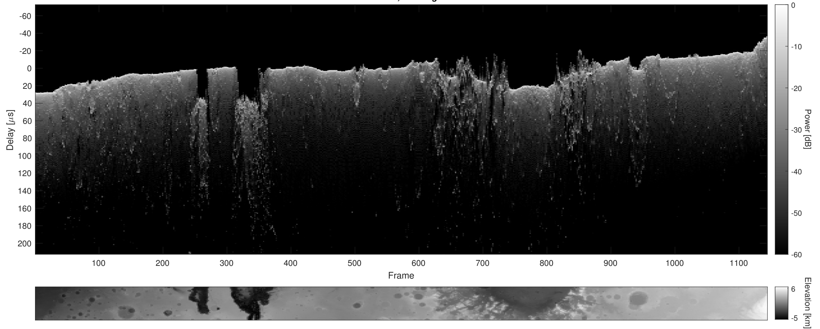
Orbit 17442, Cluttergram
