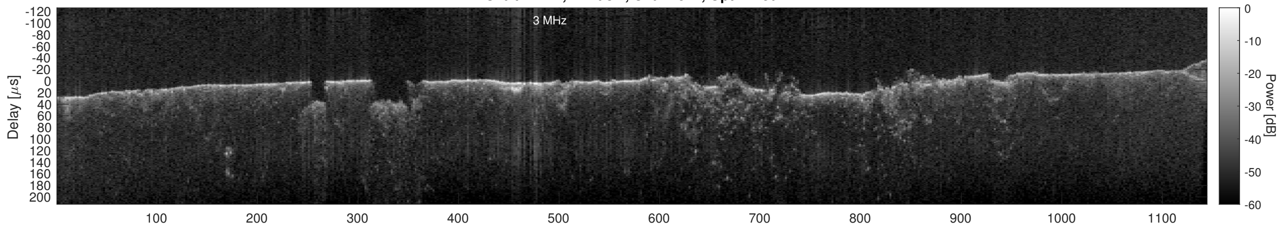
Orbit 17442, Cluttergram
