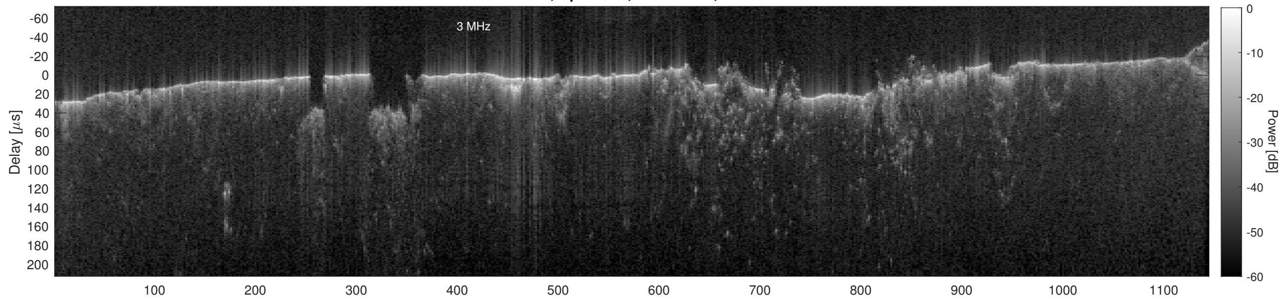
Orbit 17442, Cluttergram
