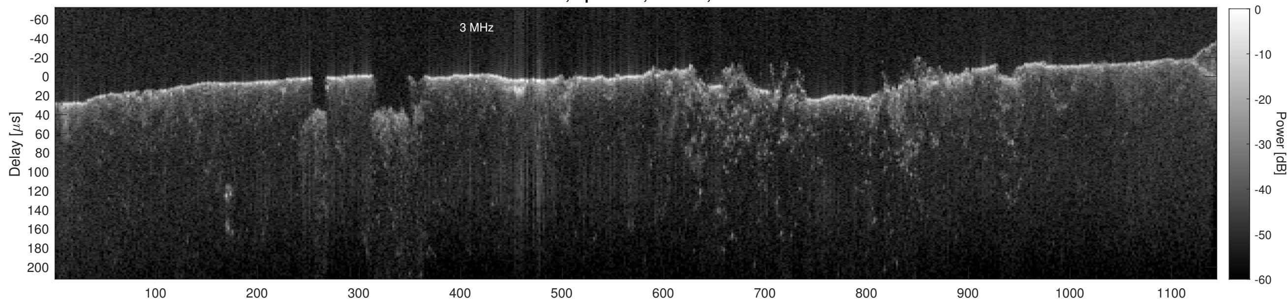
Orbit 17442, Cluttergram
