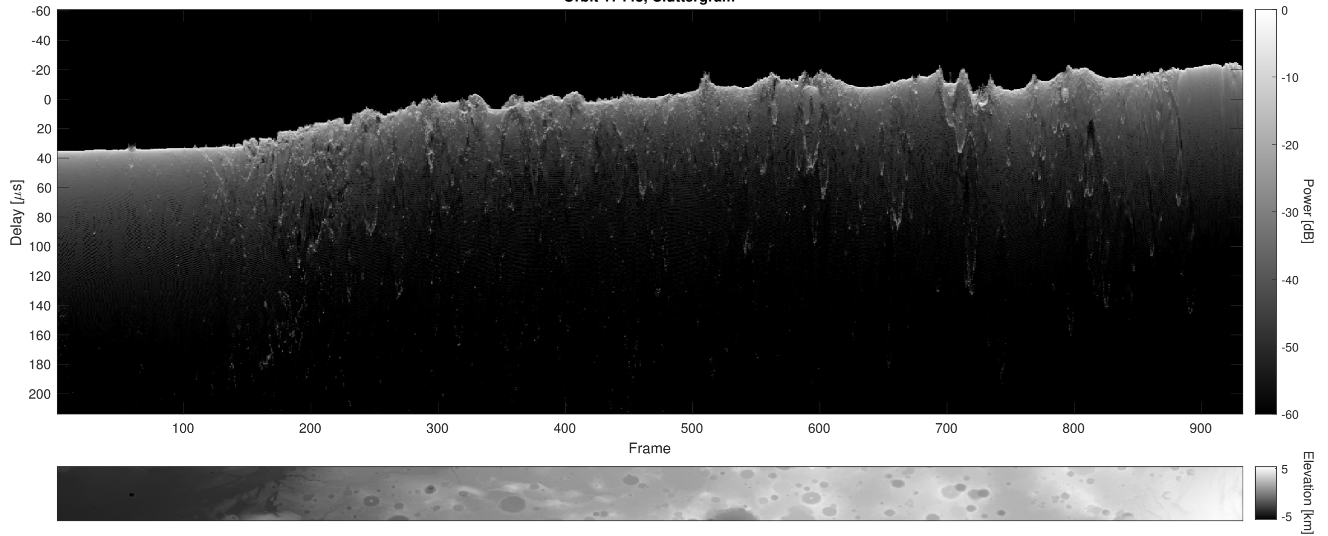
Orbit 17443, Cluttergram
