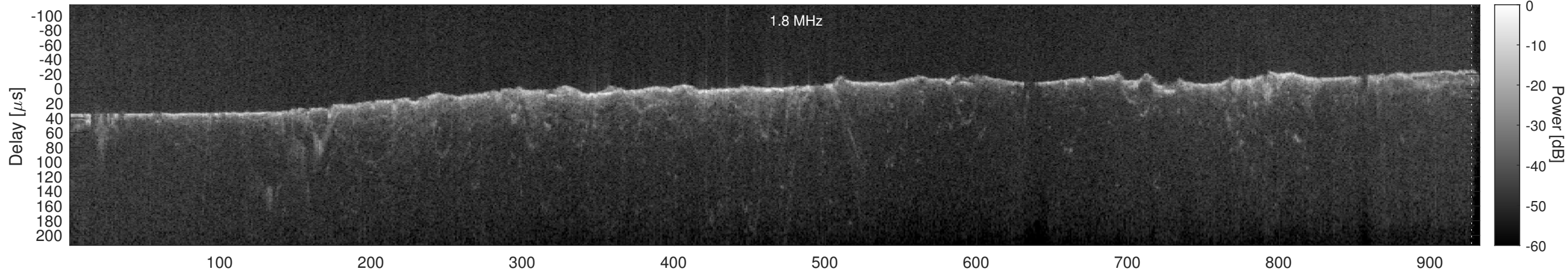
Orbit 17443, Cluttergram
