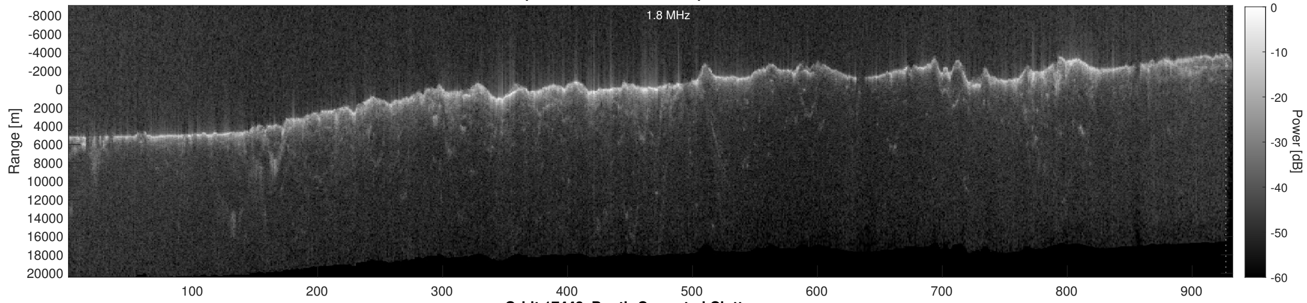
Orbit 17443, Depth-Corrected Cluttergram
