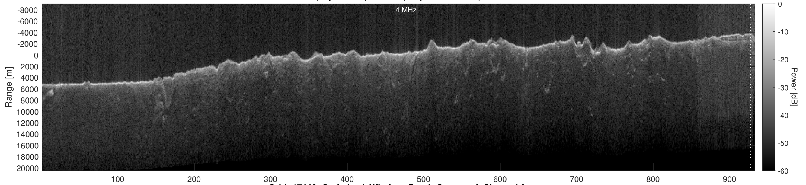
Orbit 17443, Optimized, Window, Depth-Corrected, Channel 2
