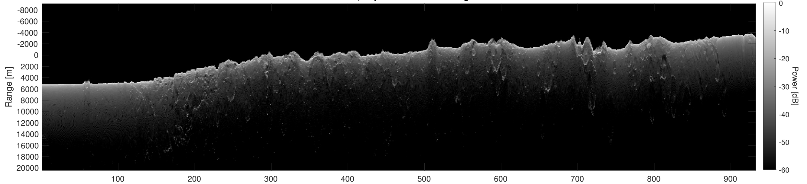
Orbit 17443, Depth-Corrected Cluttergram
