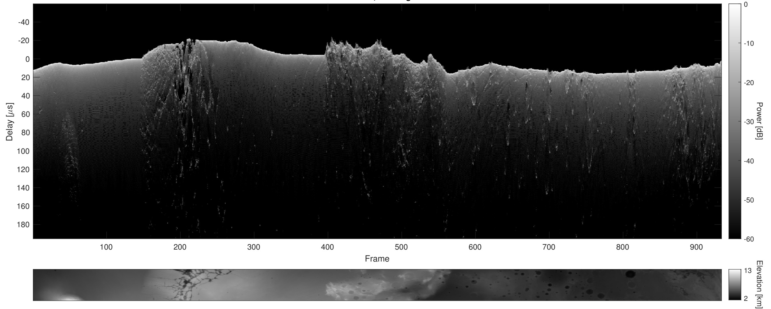
Orbit 17446, Cluttergram
