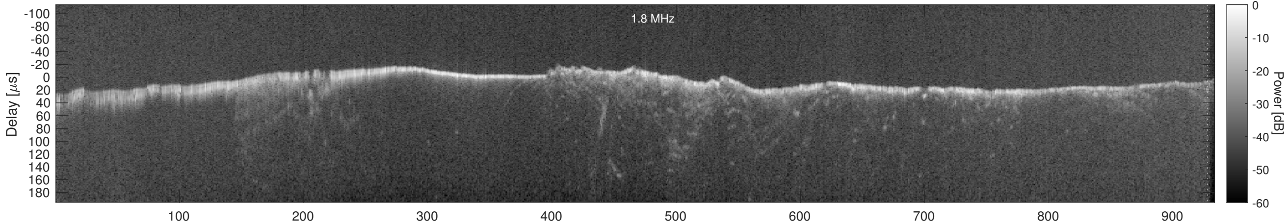
Orbit 17446, Window, Channel 2, Chapman
