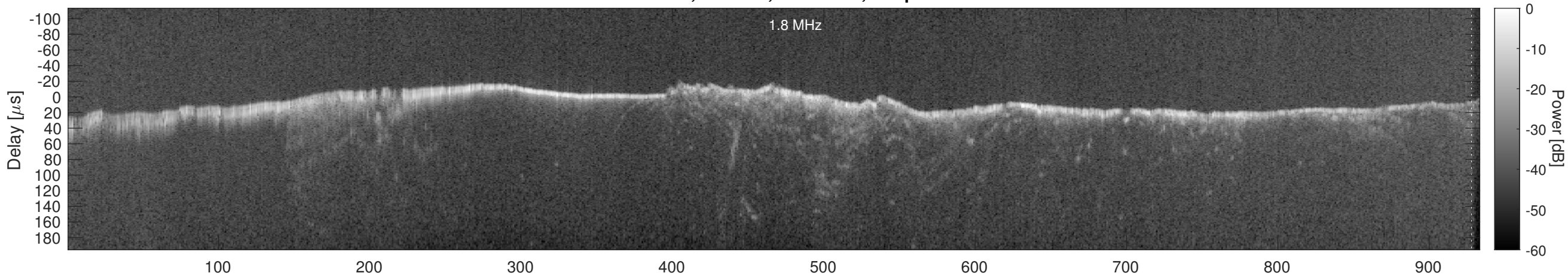
Orbit 17446, Window, Channel 2, Optimized
