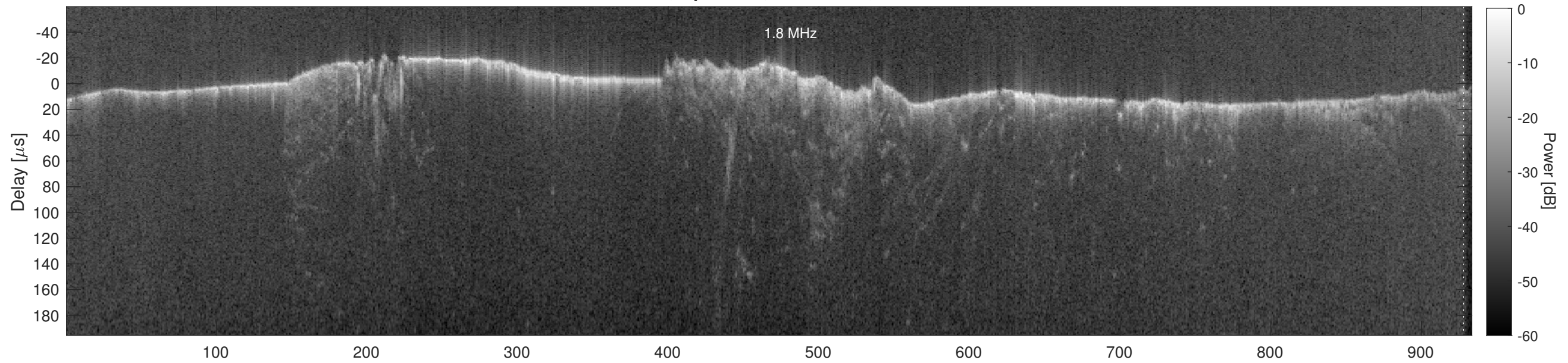
Orbit 17446, Cluttergram
