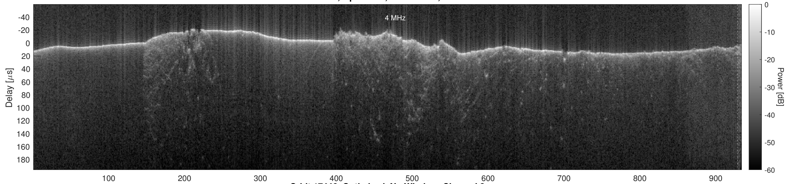
Orbit 17446, Optimized, No Window, Channel 2
