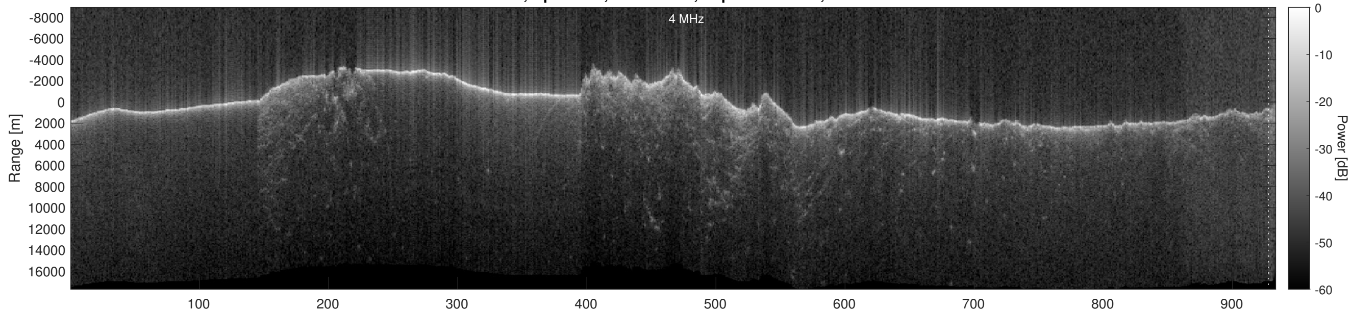
Orbit 17446, Optimized, No Window, Depth-Corrected, Channel 2
