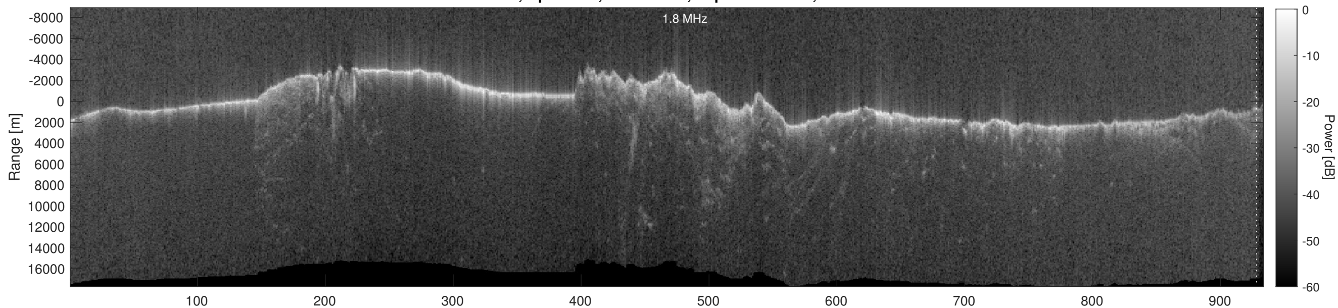
Orbit 17446, Depth-Corrected Cluttergram
