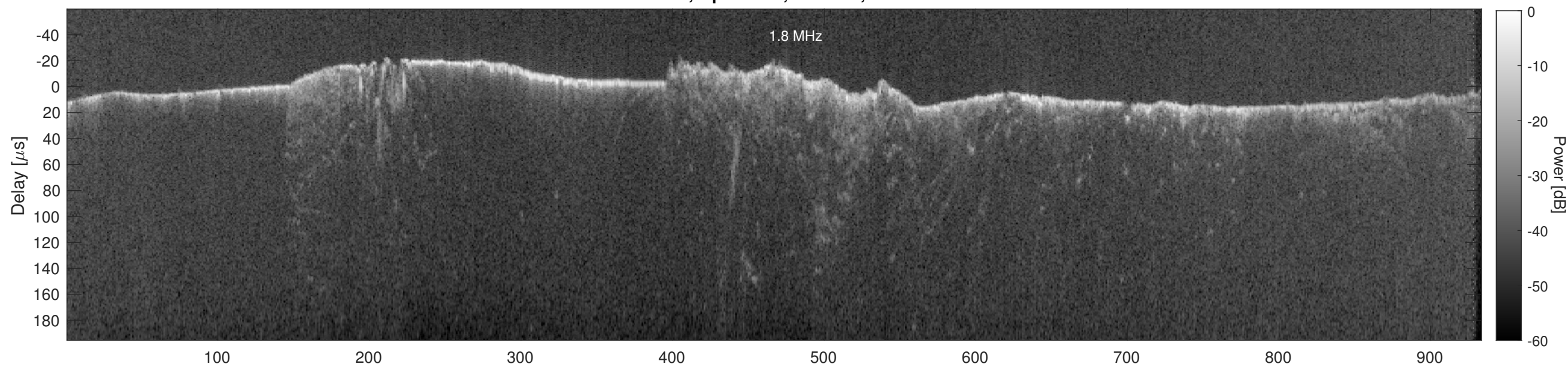
Orbit 17446, Cluttergram
