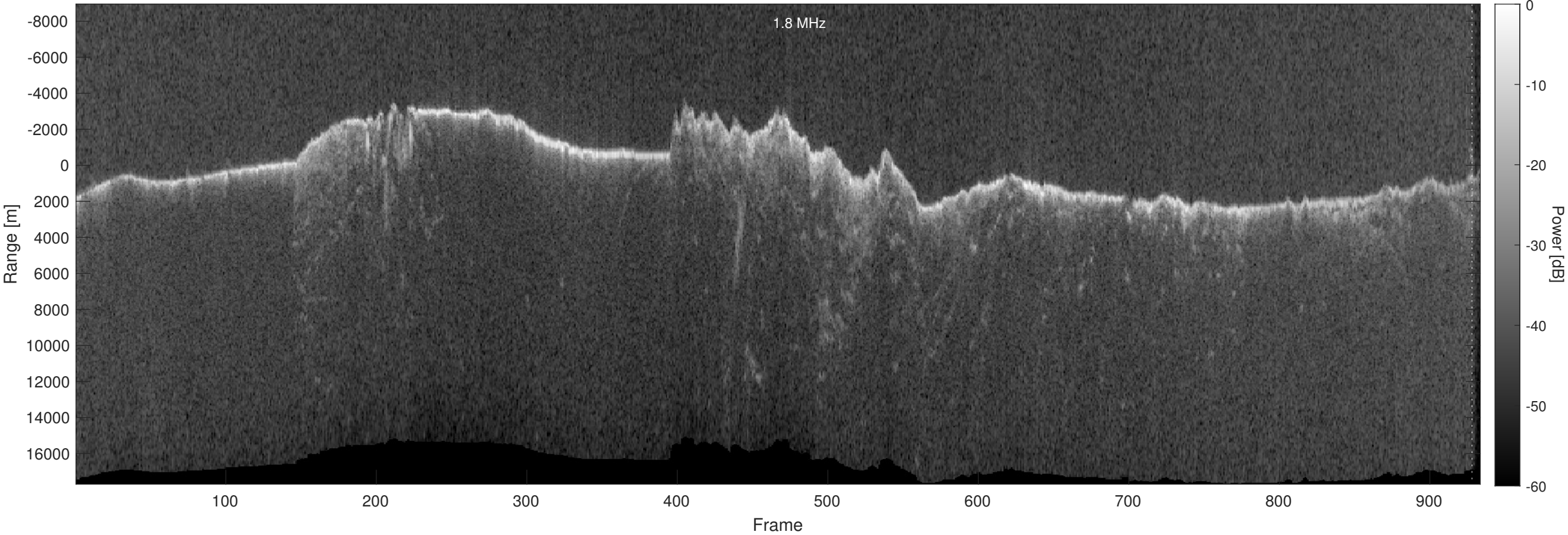
Orbit 17446, Optimized, Window, Depth-Corrected, Channel 2
