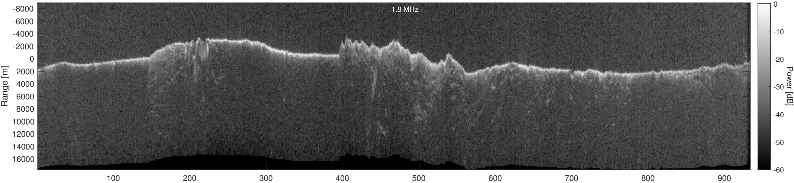
Orbit 17446, Depth-Corrected Cluttergram
