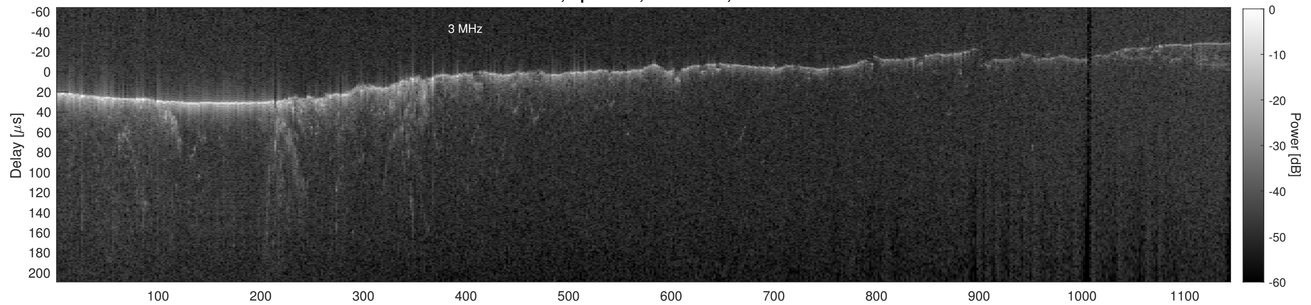
Orbit 17447, Cluttergram
