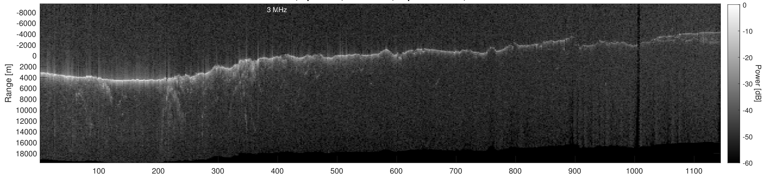
Orbit 17447, Depth-Corrected Cluttergram
