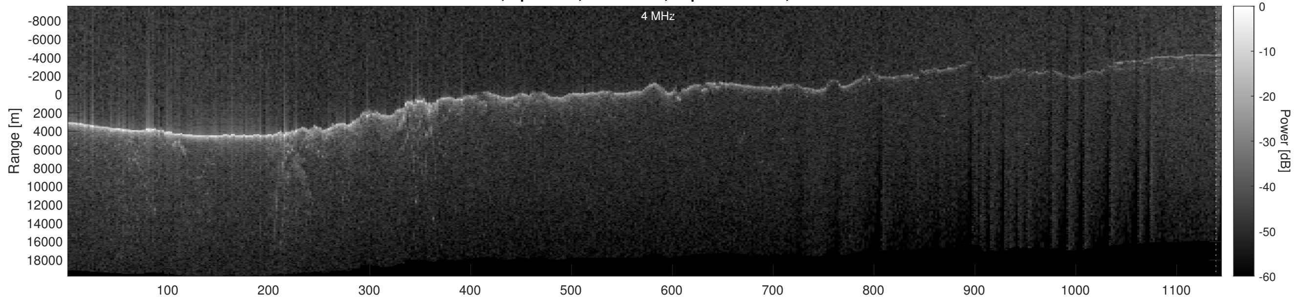
Orbit 17447, Optimized, No Window, Depth-Corrected, Channel 2
