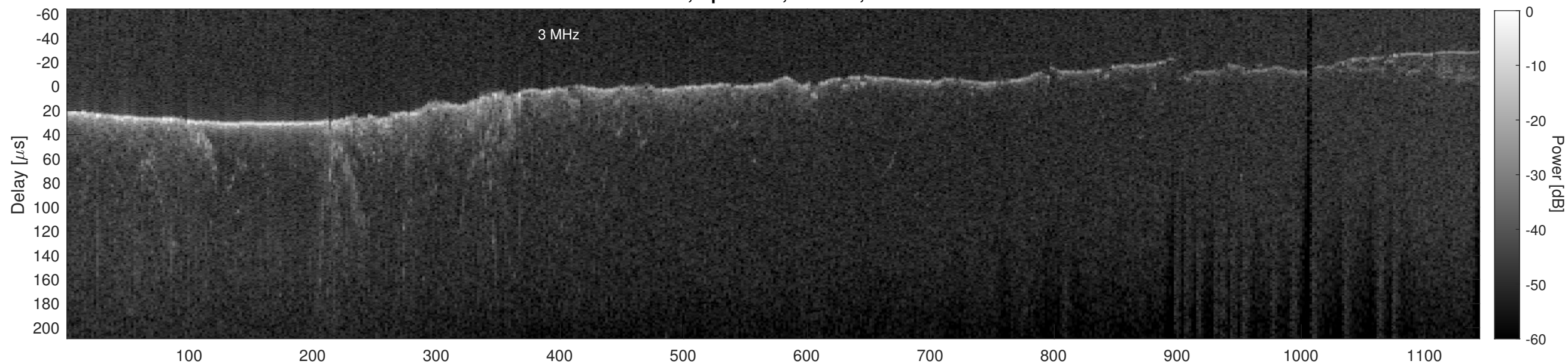
Orbit 17447, Cluttergram
