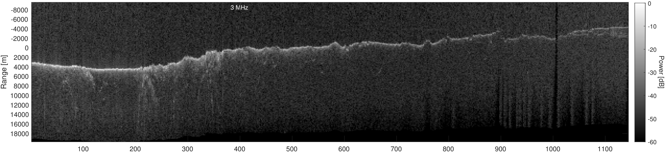
Orbit 17447, Depth-Corrected Cluttergram
