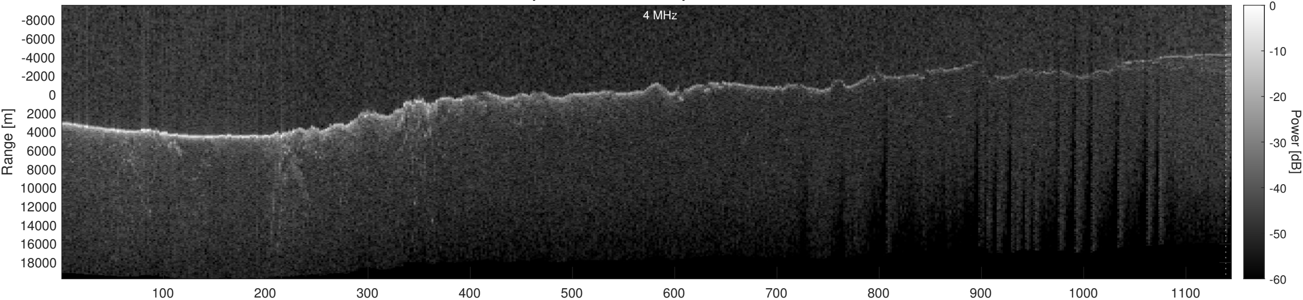
Orbit 17447, Optimized, Window, Depth-Corrected, Channel 2
