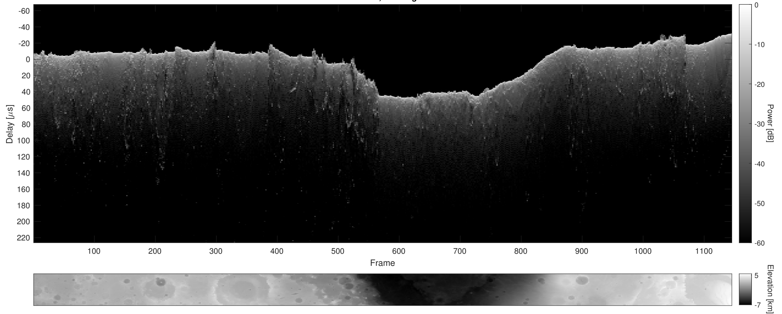
Orbit 17448, Cluttergram
