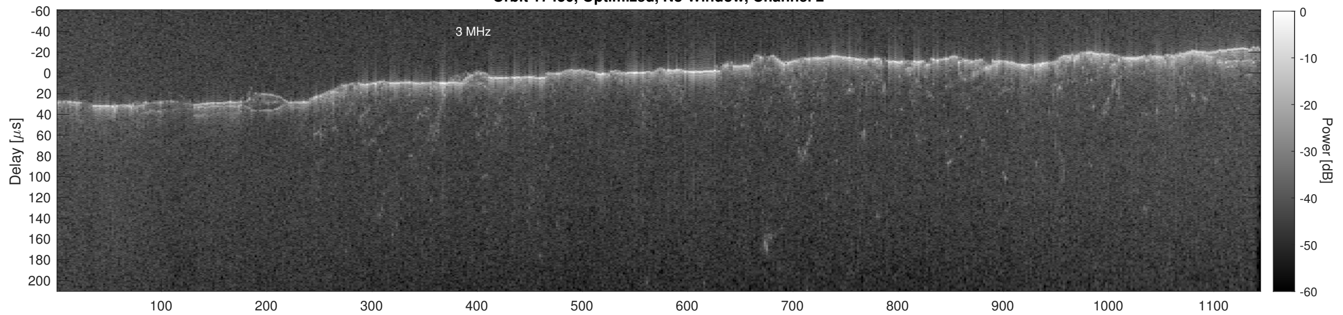
Orbit 17450, Cluttergram
