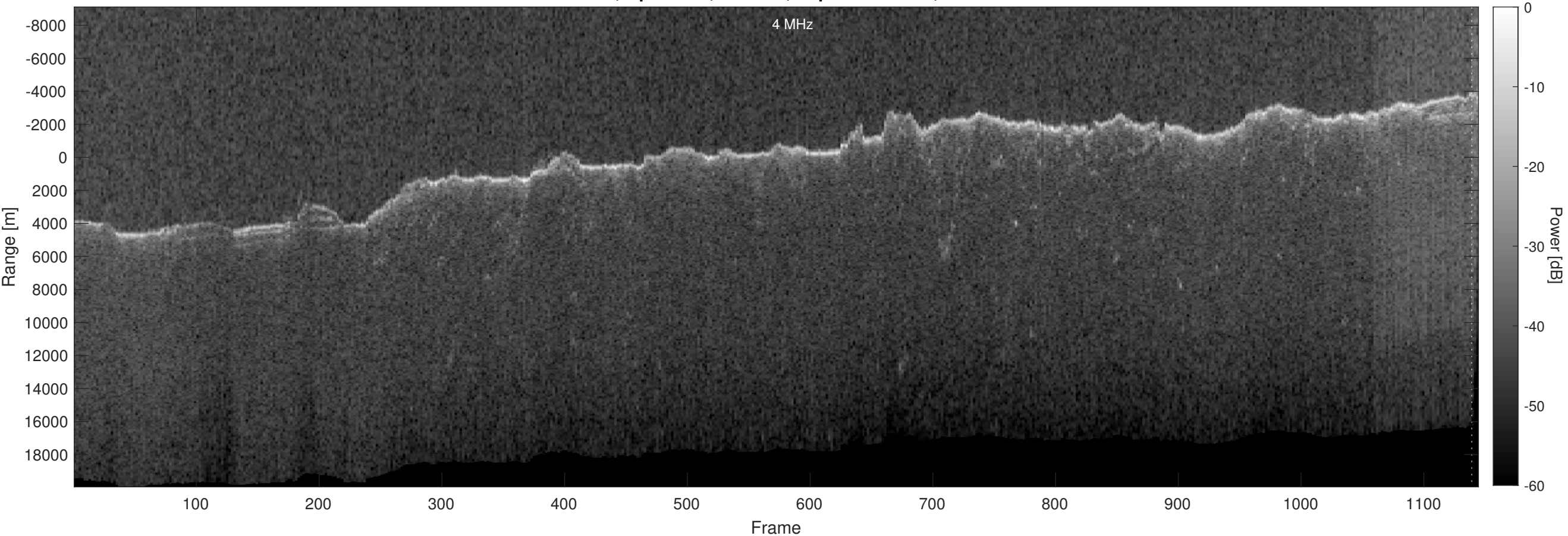
Orbit 17450, Optimized, Window, Depth-Corrected, Channel 2
