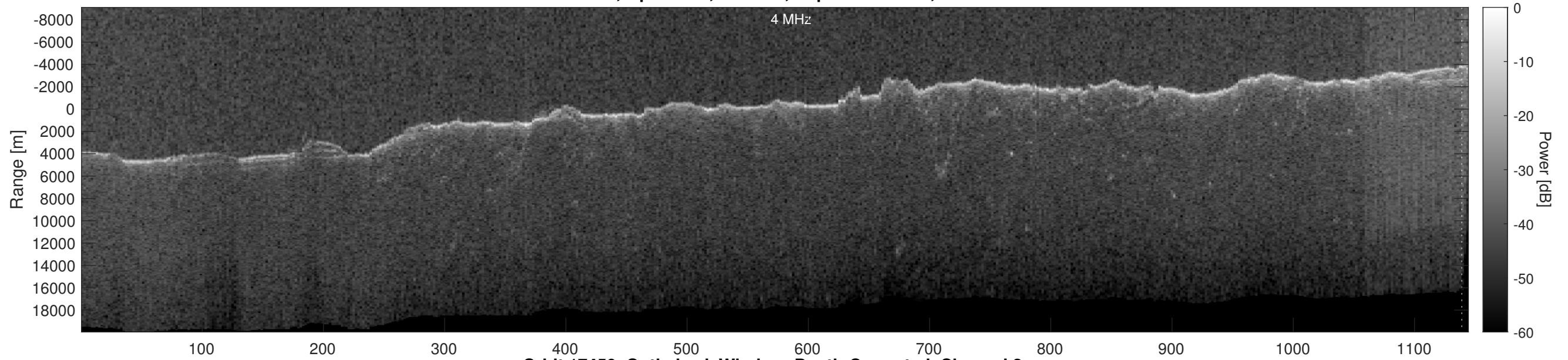
Orbit 17450, Optimized, Window, Depth-Corrected, Channel 2
