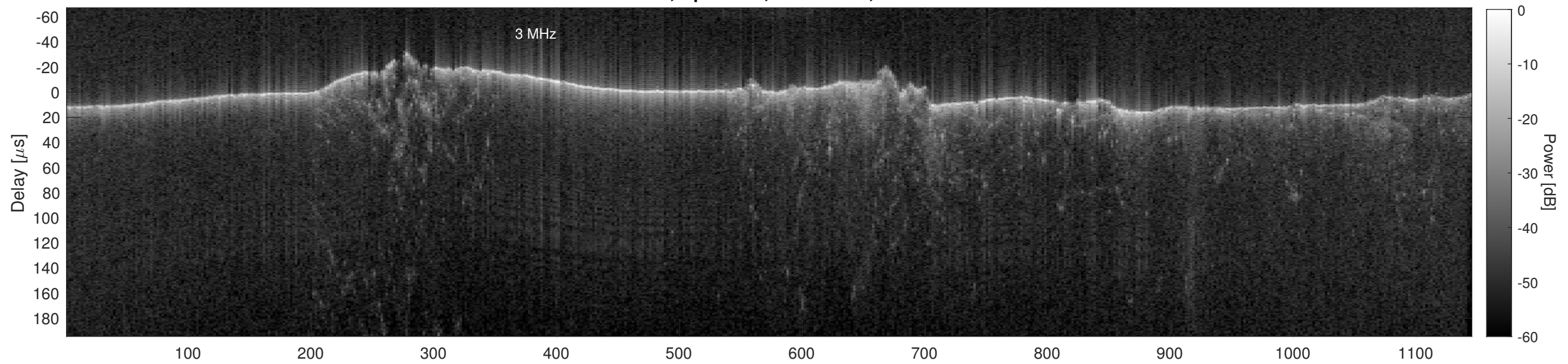
Orbit 17453, Cluttergram
